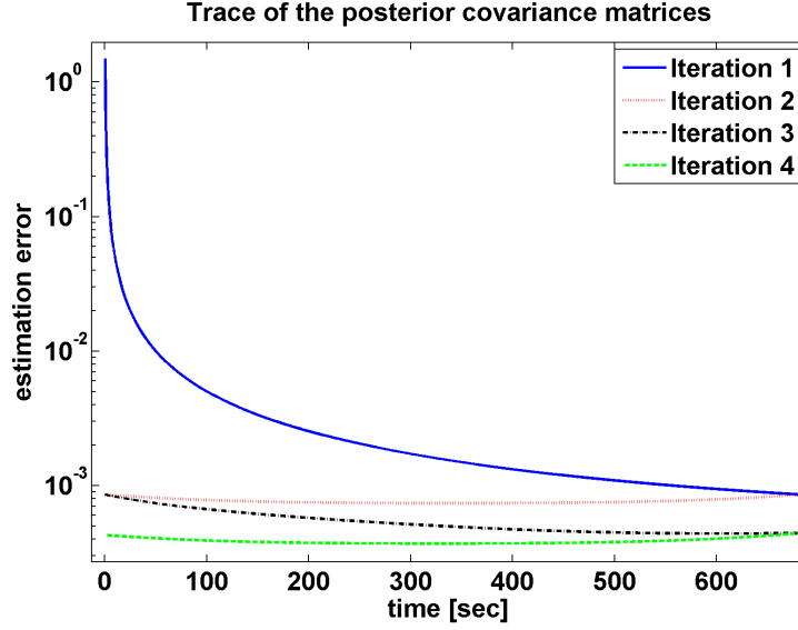
Figure 8.5: The trace of the posteriori matrices as a function of time in each iteration.
