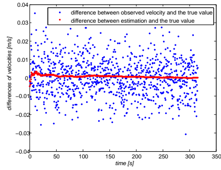
Figure 3.2: Noise suppression in the Doppler velocity measurements.
