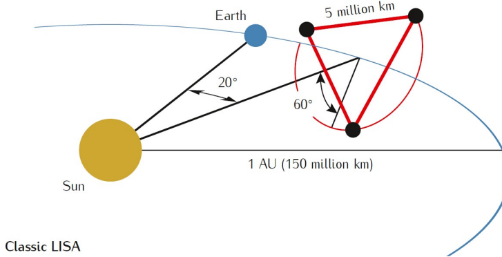
Figure 1.10: Orbits and configuration of classic LISA [78]. [Image: S. Barke].
