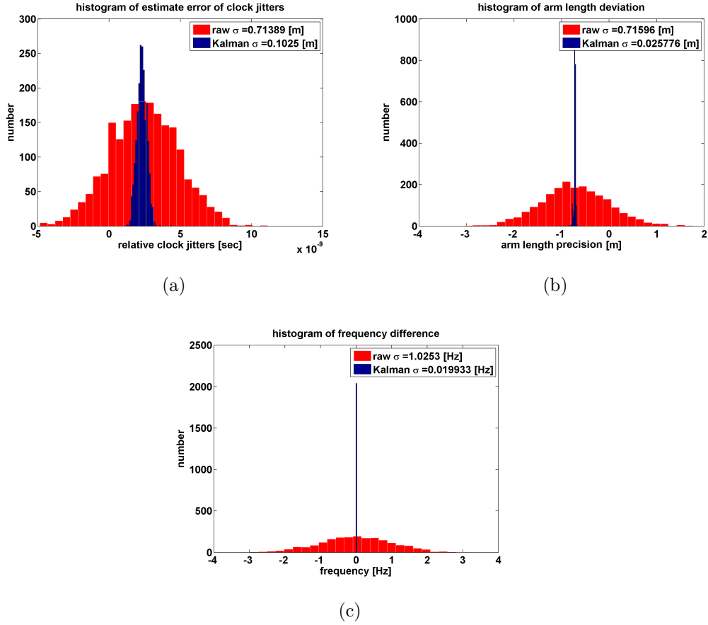
Figure 9.12: Application of the Kalman filter with the effective system dynamics to simulated LISA measurements with unknown jittering time stamps. (a). Histograms of estimation errors of relative clock jitters. (b). Histograms of estimation errors of arm lengths. (c). Histograms of estimation errors of relative frequency jitters.
