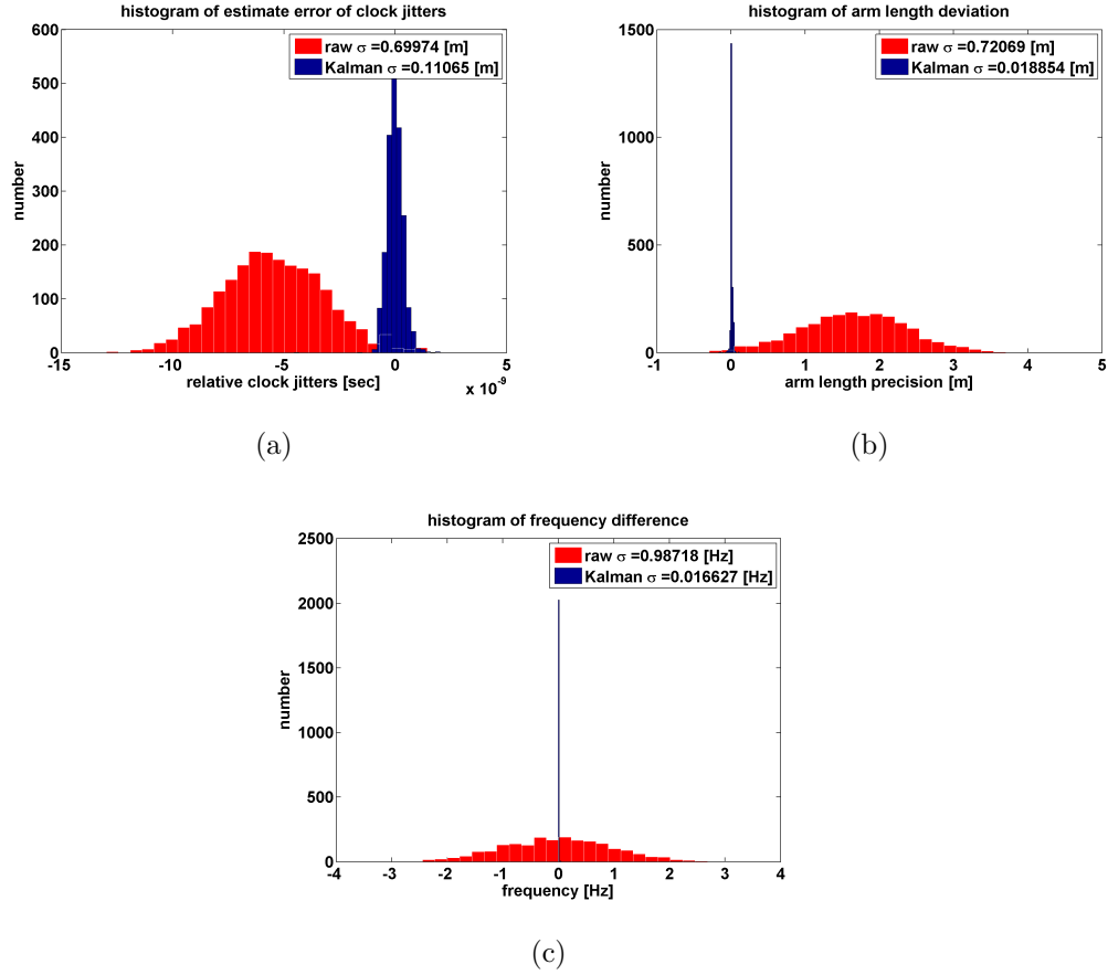
Figure 9.14: Application of the interpolated hybrid-extended Kalman filter with the 24-dimensional state vector to simulated LISA measurements with unknown jittering time stamps. (a). Histograms of estimation errors of relative clock jitters. (b). Histograms of estimation errors of arm lengths. (c). Histograms of estimation errors of relative frequency jitters.
