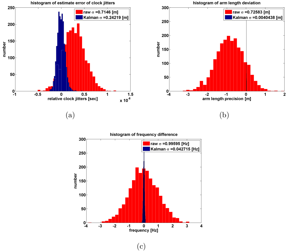
Figure 9.16: Application of the interpolated iterative Kalman filter with the fitted three-pole clock model to simulated LISA measurements with unknown jittering time stamps. (a). Histograms of estimation errors of relative clock jitters. (b). Histograms of estimation errors of arm lengths. (c). Histograms of estimation errors of relative frequency jitters.
