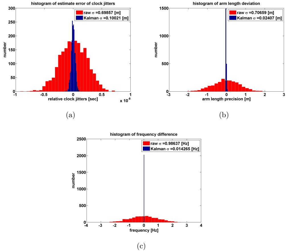
Figure 8.3: Histograms of the estimation errors of a hybrid-extended Kalman filter with a phenomenological polynomial system model in (a) relative clock jitters (b) arm lengths and (c) relative frequency jitters for the laser link from S/C 2 to S/C 1.
