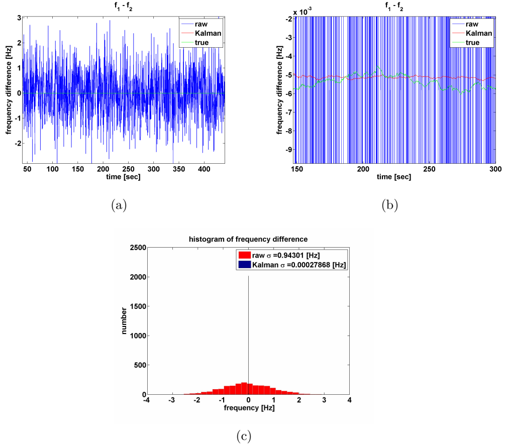
Figure 5.10: Plots of USO frequency differences. Fig. (a) shows the raw measurements, Kalman filter estimates and the true values of frequency differences between the USO in S/C 1 and the USO in S/C 2. The Kalman filter estimates are so good that they overlap with the true values. Fig. (b) is a zoomed-in plot of Fig. (a). The true USO frequency differences and the Kalman filter estimates can clearly be seen in this figure. Fig. (c) shows the histograms of the deviations of the raw measurements and the Kalman filter estimates from the true values.
