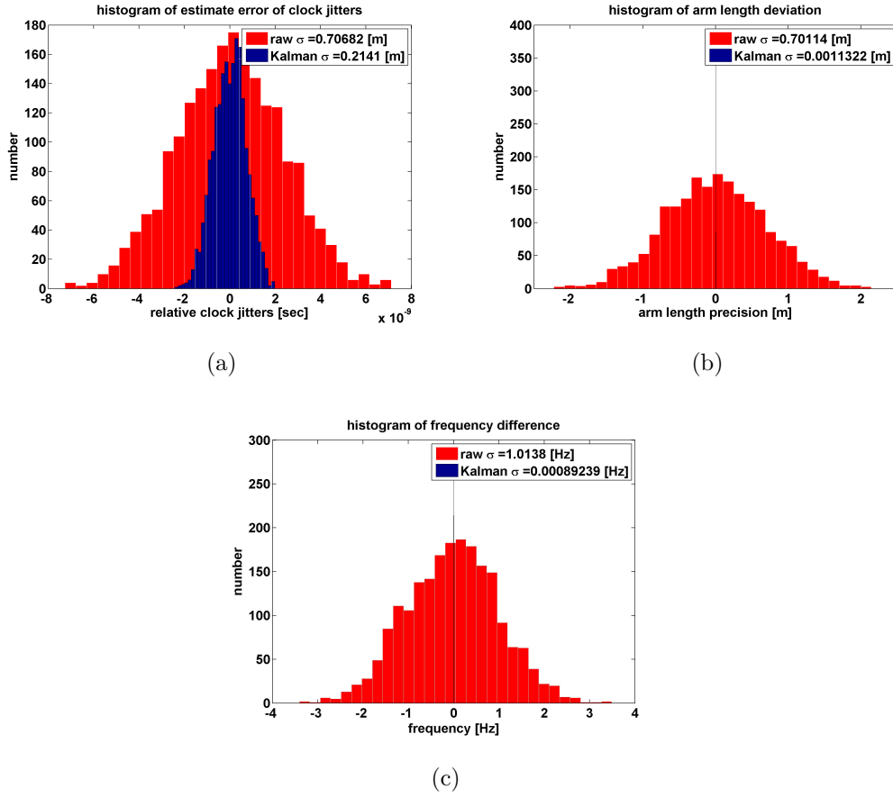
Figure 8.6: Histograms of the posteriori estimation errors after two iterations in (a) relative clock jitters (b) arm lengths and (c) relative frequency jitters for the laser link from S/C 2 to S/C 1.
