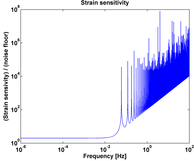
Figure 1.15: Strain sensitivity of a single-link one-way detector with an arm length of L = 5 \times 10^9 \text{m} . Here we assume the sensitivity of the detector is limited only by white noise.
