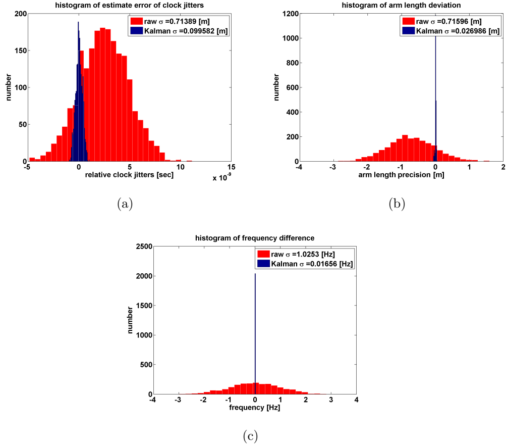
Figure 9.15: Application of the interpolated Kalman filter with the effective system model to simulated LISA measurements with unknown jittering time stamps. (a). Histograms of estimation errors of relative clock jitters. (b). Histograms of estimation errors of arm lengths. (c). Histograms of estimation errors of relative frequency jitters.
