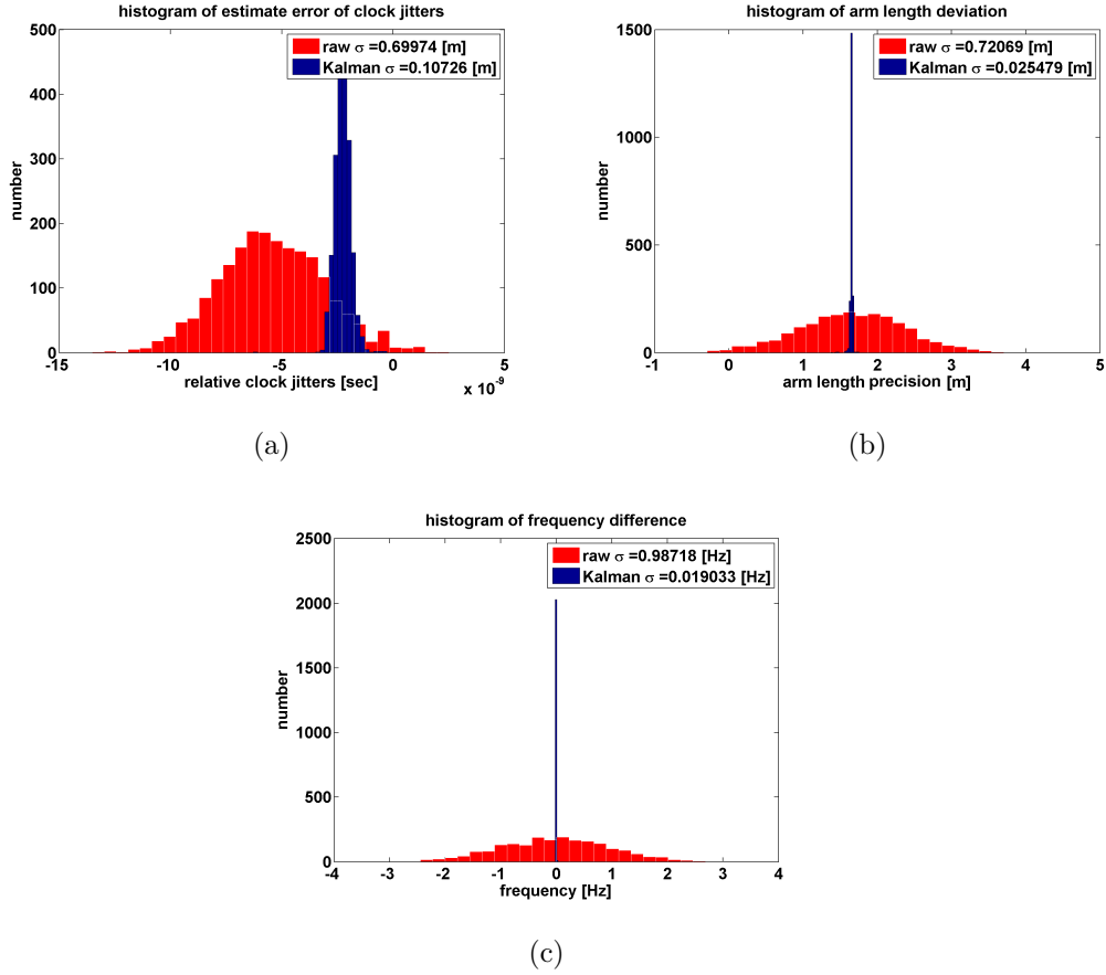
Figure 9.11: Application of the hybrid-extended Kalman filter with the 24-dimensional state vector to simulated LISA measurements with unknown jittering time stamps. (a). Histograms of estimation errors of relative clock jitters. (b). Histograms of estimation errors of arm lengths. (c). Histograms of estimation errors of relative frequency jitters.
