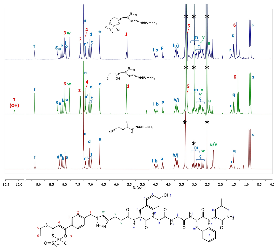
Figure 4. ^1\text{H} NMR spectra (400 MHz, \text{DMSO-d}_6 ) of Pt(II) complex 32 (top), the ligand with triazole linker 31 (middle) and the starting material, alkyne-derived Leu 5 –Enk 26 (bottom). The signal of Pt-coordinated DMSO is not witnessed in the spectrum of 32 due to a gradual exchange by \text{DMSO-d}_6 .
