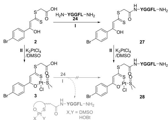
Scheme 5. Synthetic approaches towards (O,S)Pt bioconjugates through amide bond formation. When subjecting 3 to standard coupling conditions, 28 could not be isolated. Instead, (Enk–O,S)Pt complexes are formed with a mixture of monodentate ligands X/Y. Reaction conditions: I, acid ( 2 or 3 )/ 24 (1.1:1 equiv.), 1.1 equiv. TBTU, 2.3 equiv. DiPEA, DMF, r.t., 2 h. II [i] NaOAc·3 H 2 O, [ii] 1.1 equiv. K 2 PtCl 4 /DMSO, THF/H 2 O, r.t.
