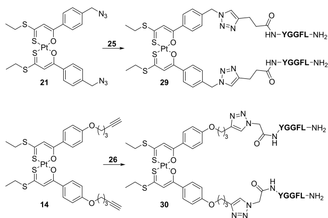
Scheme 6. Bioconjugation of azide and alkyne containing (O,S) 2 Pt bischelates 21 and 14 with the complementary Enk derivatives 25 resp. 26 by CuAAC. Reaction conditions: azide/alkyne (1 : 1 molar ratio), 0.2 equiv. CuSO 4 ·5H 2 O, 0.4 equiv. sodium ascorbate, THF/H 2 O, r.t.
