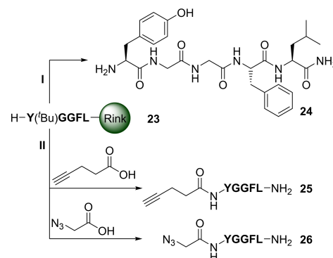
Scheme 4. Solid-phase peptide syntheses of Leu 5 –Enk derivatives 24–26 . Reaction conditions: I, TFA/H 2 O/TES (95:2.5:2.5 v/v), r.t., 2 h. II, [i] 4 equiv. acid (pentynoic acid or azidoacetic acid), 4 equiv. 1-hydroxybenzotriazole (HOBt), 3.8 equiv. N,N,N',N' -tetramethyl- O -(benzotriazol-1-yl)uronium tetrafluoroborate (TBTU), 8 equiv. diisopropylethylamine (DiPEA), DMF, r.t., 2 h, [ii] TFA/H 2 O/TES (95:2.5:2.5 v/v), r.t., 2 h.
