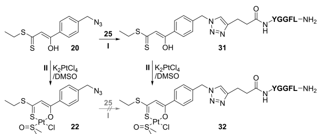
Scheme 7. Pathways towards (Enk-O,S)Pt complex 32 via CuAAC. Reaction conditions: I, [i] azide/alkyne (1 : 1 molar ratio), 1.2 equiv. CuSO 4 ·5H 2 O, 2.4 equiv. sodium ascorbate, [ii] 2.5 equiv. Na 2 EDTA, THF/H 2 O, r.t. II [i] NaOAc·3 H 2 O, [ii] 1.1 equiv. K 2 PtCl 4 /DMSO, THF/H 2 O, r.t.
