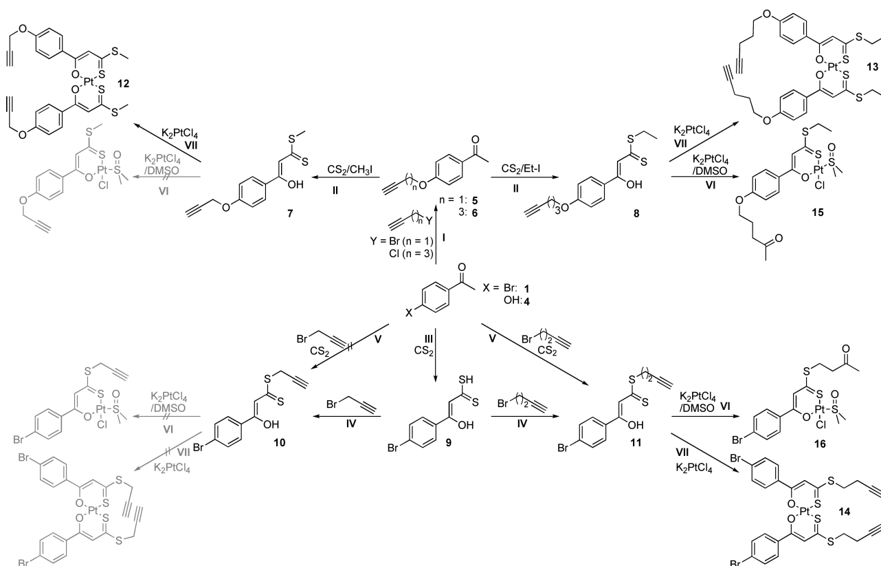
Scheme 2. Synthesis of \beta -hydroxydithiocinnamic esters with a terminal alkyne at the aromatic (7, 8) or dithio subsite (10, 11) via functionalized acetophenones as well as coordination reactions towards mono- and bisfunctional Pt(II) complexes. Reaction conditions: I, 1.5 equiv. base ( K_2CO_3 or CS_2CO_3/KI ), 1.1 equiv. alkynyl halide (propargyl bromide or pentynyl chloride), acetonitrile, reflux, 20 h. II, [i] 2.5–3 equiv. KO^tBu , 1.4 equiv. CS_2 , -78^\circ C to r.t., 4 h, [ii] 1 equiv. alkyl iodide, r.t. 15 h, [iii] H^+/H_2O . III, [i] 2 equiv. KO^tBu , 1.4 equiv. CS_2 , Et_2O , -78^\circ C to r.t., 15 h [ii] H^+/H_2O . IV, 1 equiv. ^nBu_4NOH , 1 equiv. alkynyl bromide, CHCl_3 , r.t., 2 h. V, [i] 2 equiv. KO^tBu , 1.4 equiv. CS_2 , -78^\circ C to r.t., 4 h, [ii] 0.9 equiv. alkynyl bromide, r.t. 15 h, [iii] H^+/H_2O . VI [i] NaOAc \cdot 3 H_2O , [ii] 0.5 equiv. K_2PtCl_4 , THF/ H_2O , r.t. VII [i] base ( NaOAc \cdot 3 H_2O or NaH ), [ii] 1.1 equiv. K_2PtCl_4 /DMSO, THF/ H_2O , r.t.
