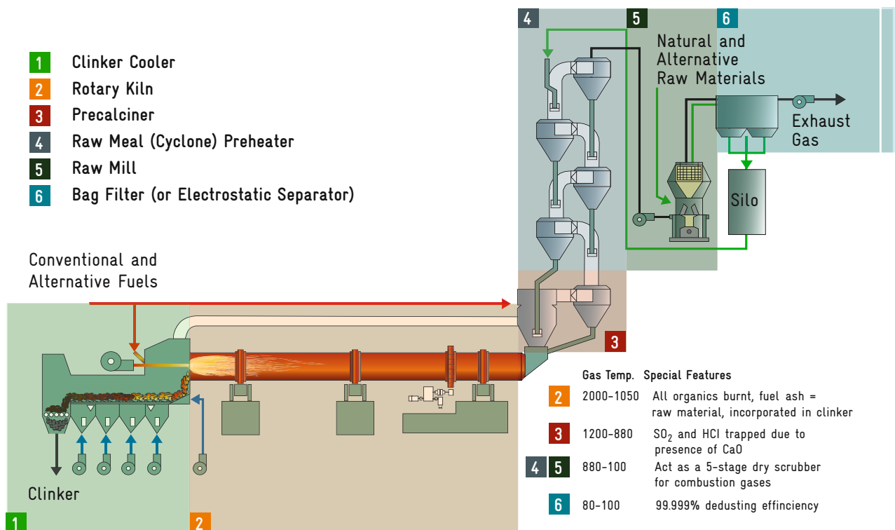
Figure 7: Components of a cement kiln form the type pre-calculator and its special characteristics [18].
